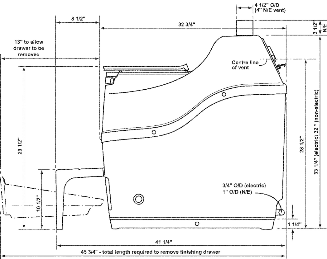
PLAN ELEVATION
